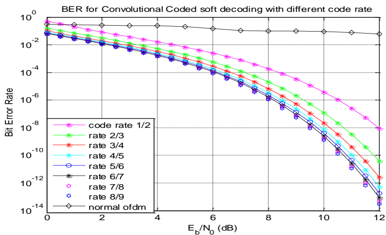
Fig.6. CC-OFDM at different code rates
