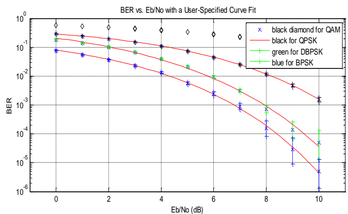
Fig.5. CC-OFDM at different modulation
