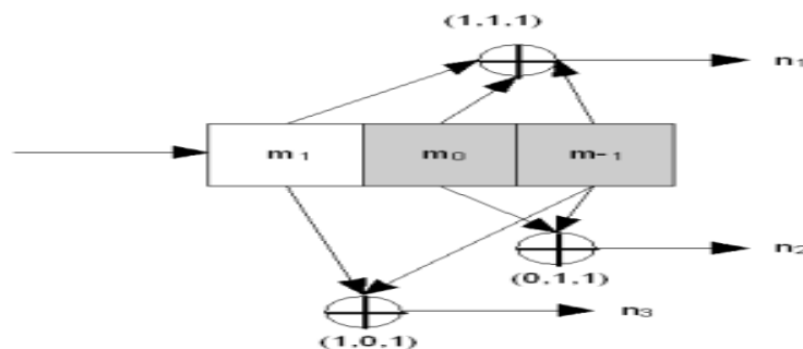
Fig 2. Rate 1/3 non-recursive CC-Encoder
