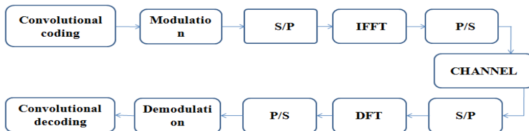
Fig.1. OFDM with Convolution Code
