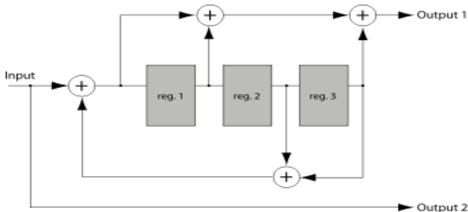
Fig.3. Rate 1/2 recursive systematic CC-encoder
