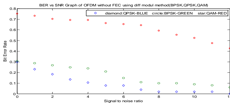
Fig 4. OFDM with different modulation methods
